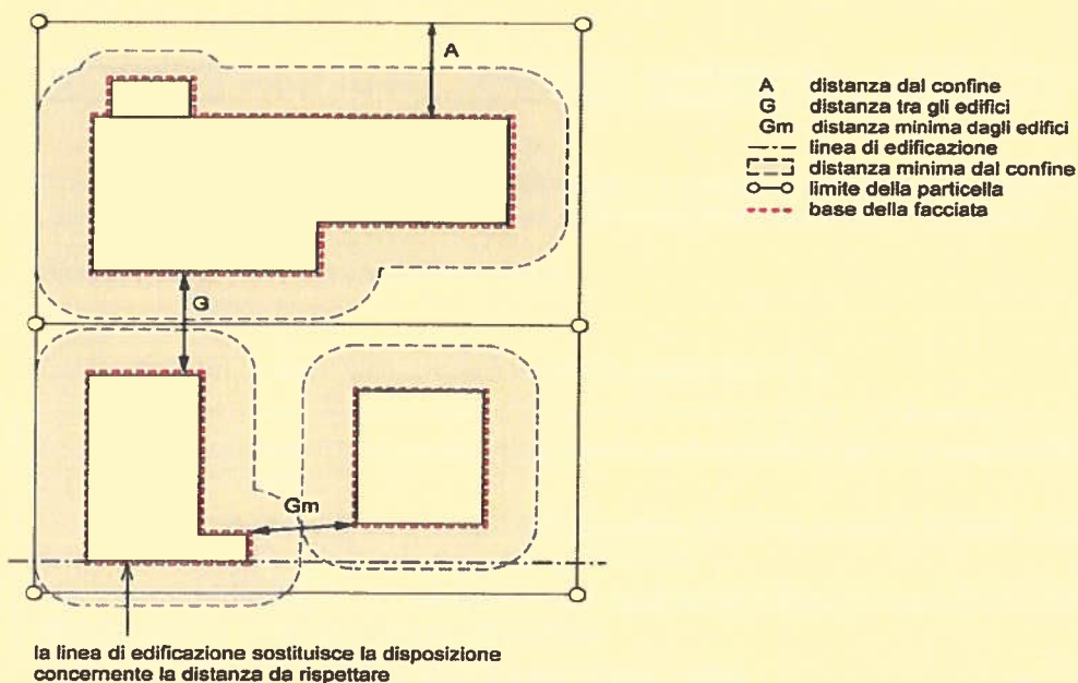
Figure 7.1 – 7.3 Distanze
